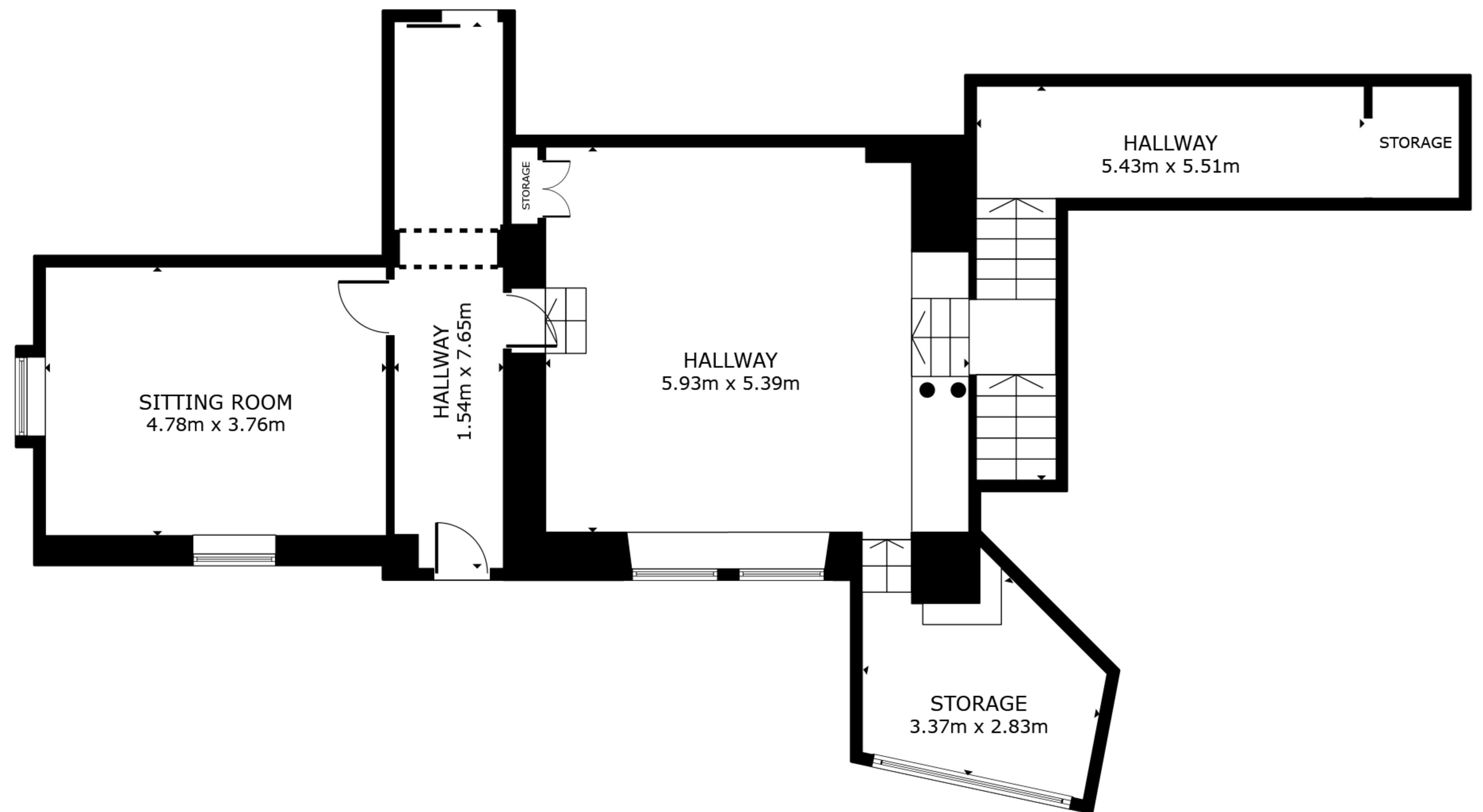
FLOOR 1
