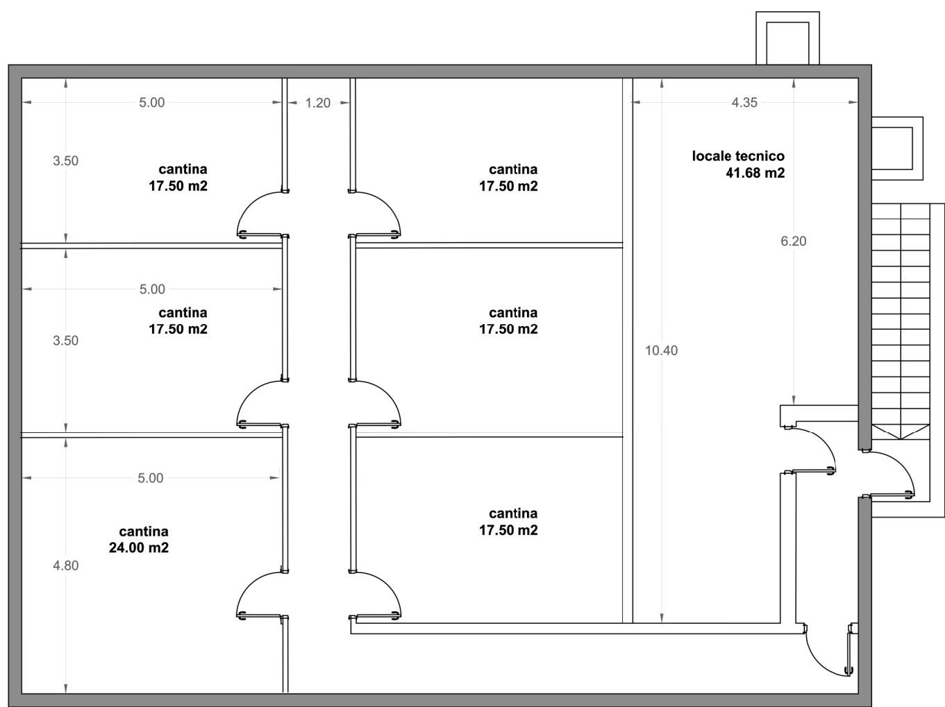
PIANO INTERRATO
