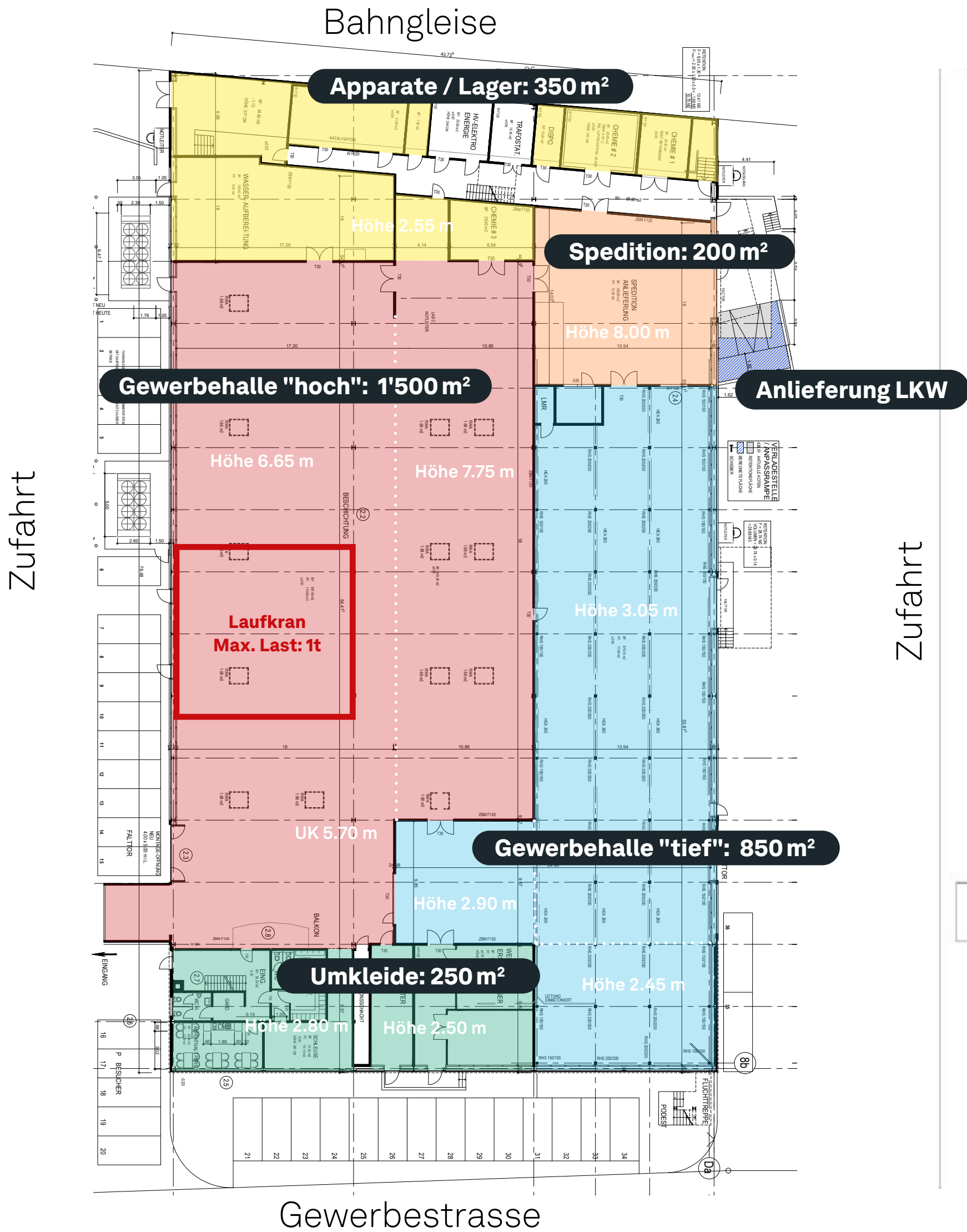
Erdgeschoss, 3'150 m²
